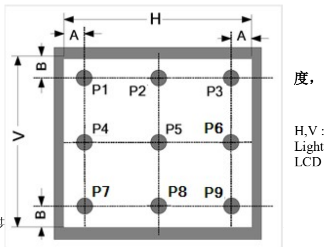
FIG.1. Measuring method for Contrast ratio, surface luminance, Luminance uniformity, CIE (x, y) chromaticity 对比度，表面亮度，均匀度，CIE坐标测试方法
