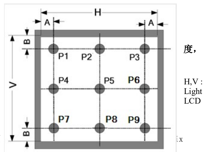
FIG.1. Measuring method for Contrast ratio, surface luminance, Luminance uniformity, CIE (x, y) chromaticity 对比度，表面亮度，均匀度，CIE坐标测试方法
