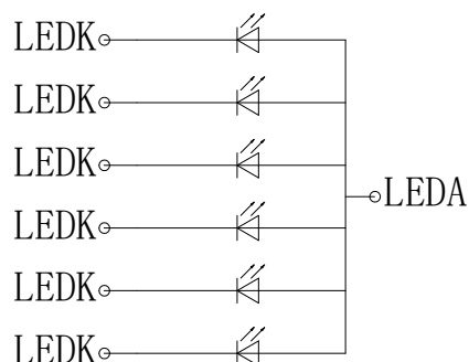
LED CIRCUIT DIAGRAM: 1S6P 6LED
