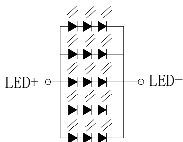
Backlight LED Circuit ( I_f=100\text{mA} , V_f=9.0\text{V}-9.9\text{V} )
