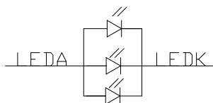
Backlight LED Circuit ( I_f=60\text{mA} , V_f=2.8\text{V}-3.6\text{V} )
