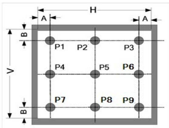
FIG. 2. The definition of Response Time 响应时间定义
