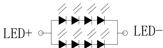
LED CIRCUIT DIAGRAM
